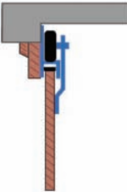
Lintel less than 100 mm / Partial fascia
