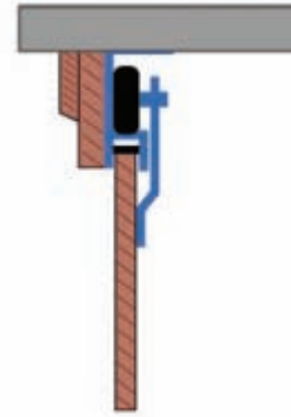
Angled corner fascia 120 mm
